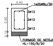
RIOSTRA R-01
