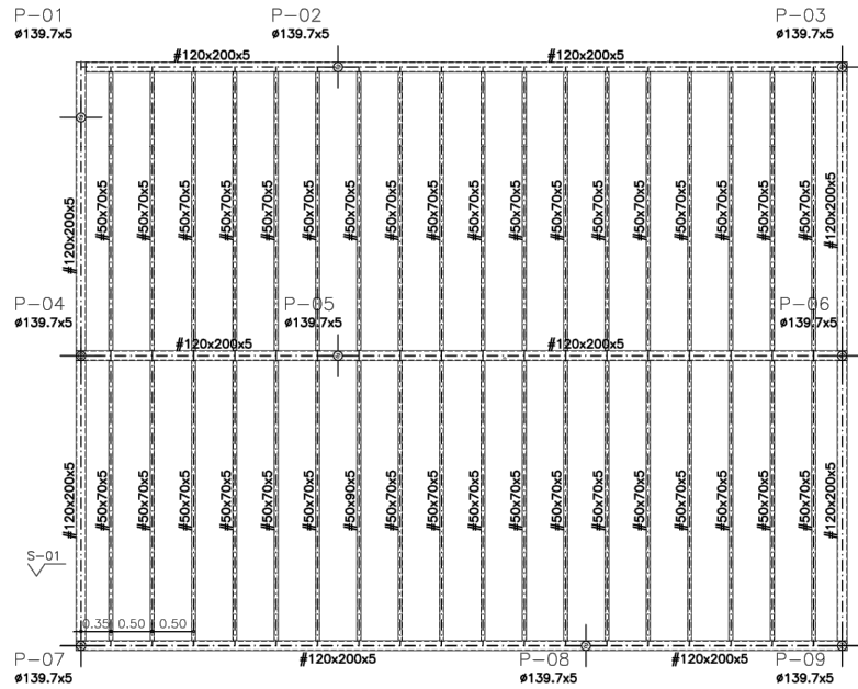
SN01_COBERTA E_A1: 1/50 ; E_A3: 1/100 GEOMETRIA
